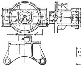
Figs. 3381-3383. Truck Center Plate Casting.
